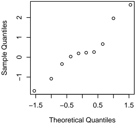
Normal Q-Q Plot A
