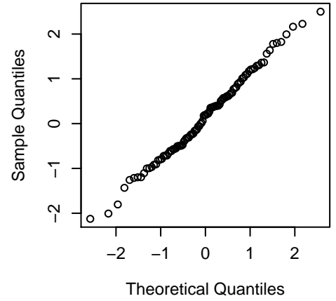
Normal Q-Q Plot G
