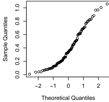
Normal Q-Q Plot D
