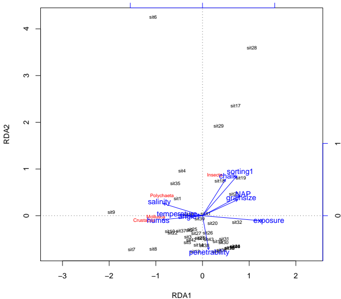
Correlation biplot
